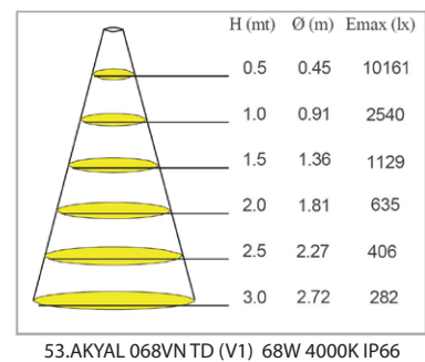
53.AKYAL 068VN TD (V1) 68W 4000K IP66
